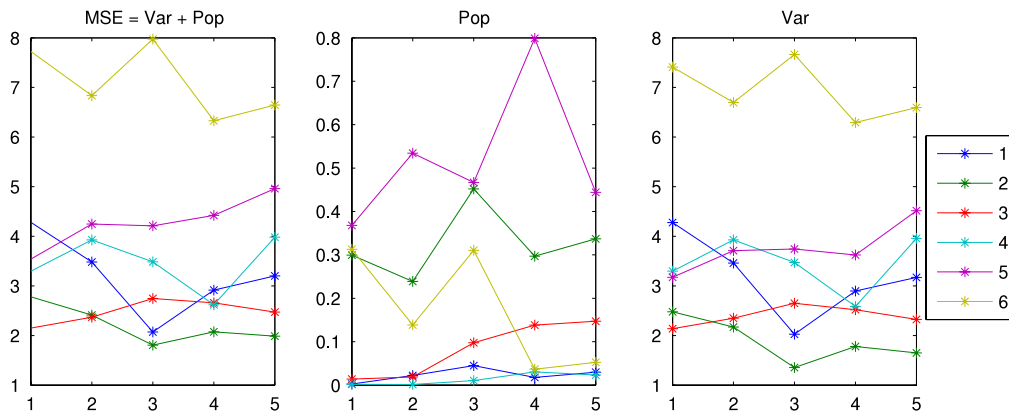
Fig. A.2. Population bias \text{Pop}(x_T^d) , variance \text{Var}(x_T^d) , and mean of squared errors \text{MSE}(x_T^d) for questions 1–6. Note, that \text{MSE}(x_T^d) is not the same as \text{MSE}(\bar{x}_T^d) from Fig. 2.
