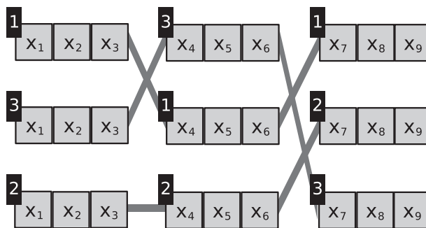
Figure 6 Product assembly in the disintegrated case: all firms are ranked (1–3) by their expected sub-product quality. Firms with the same rank contribute to one final product.
