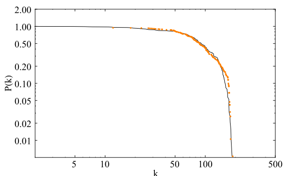
Fig. 7.7 Degree distribution in the undirected WTW (year 1995): (points) real data; (solid line) theoretical prediction of the fitness model
